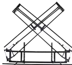
2308QJ 8 Row (3 Section) 28' Boom Assembly With 17 Nozzle W/QuickJet Diaphragm
