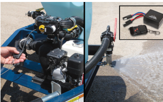
Wireless-Remote
